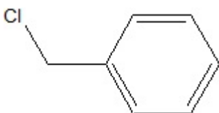
Benzyl Chloride
